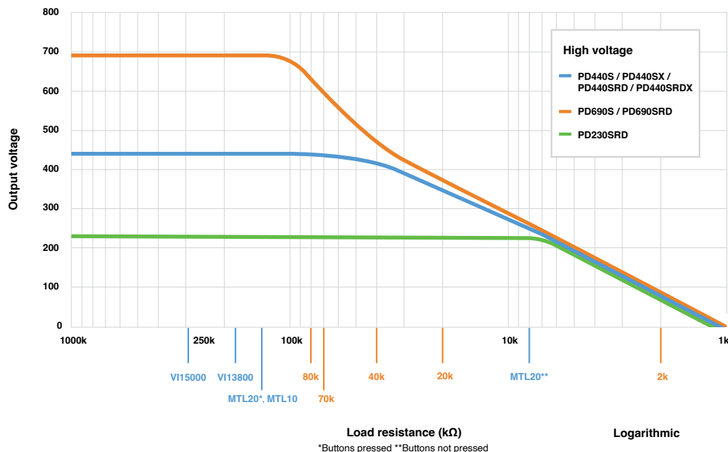
Typical output voltage AC rms vs loading (kΩ)
